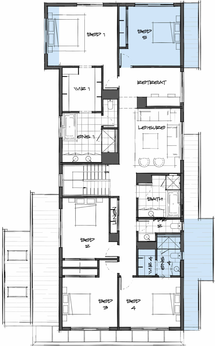
First Floor
